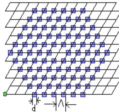
Fig.1. The cross section of PCF with a regular triangular air-hole array defined by air hole diameter d and the pitch \Lambda .
