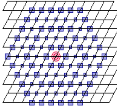
Fig.2. square hole PCF with alternate layer air-hole diameter change.
